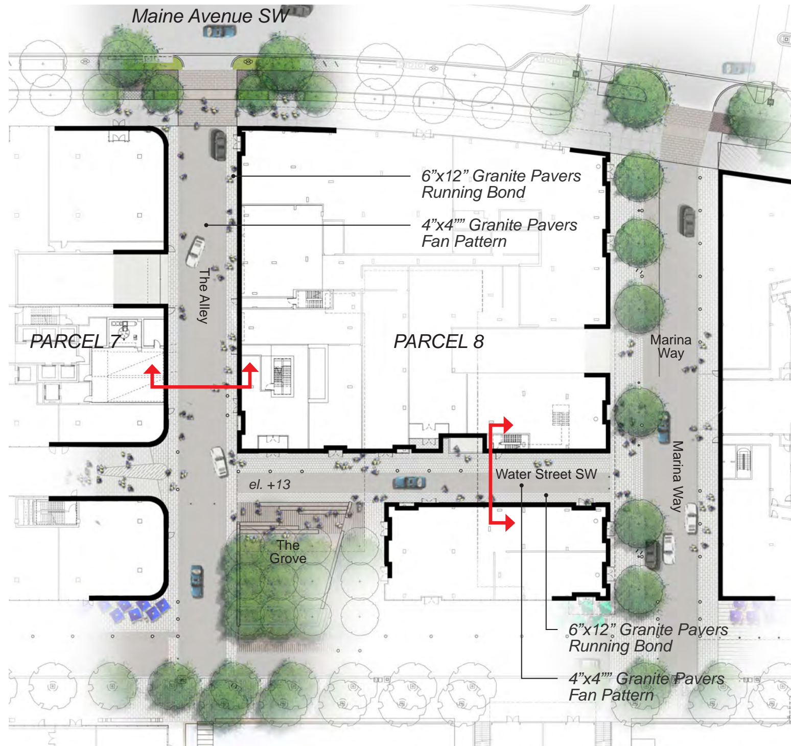
Mews Plan
